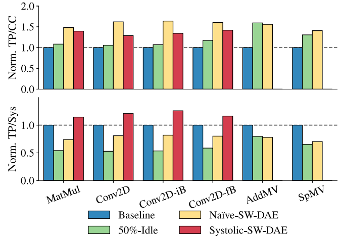
Fig. 7. Naïve and Systolic Software DAE: TP/CC = throughput per compute core; TP/Sys = overall throughput per system; MatMul showing 768 \times 768 \times 768 ; Conv2D, Conv2D-iB, and Conv2D-fB showing 32 images batch; AddMV showing 768 \times 768 ; and SpMV showing FB-Johns55. See Table II for detailed input specification.
