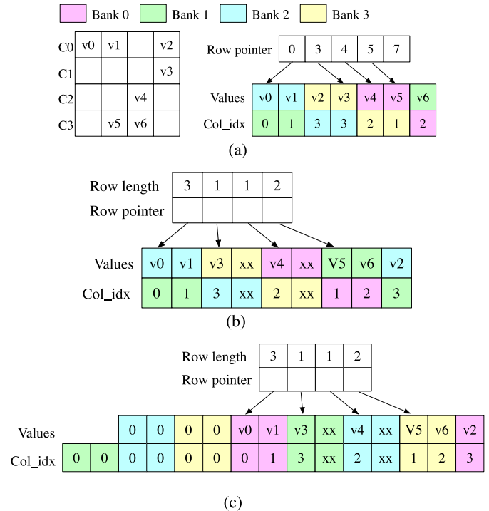
Fig. 4. CSR and CBSR sparse tensor formats. (a) CSR format. (b) CBSR format. (c) CBSR+Padding format.
